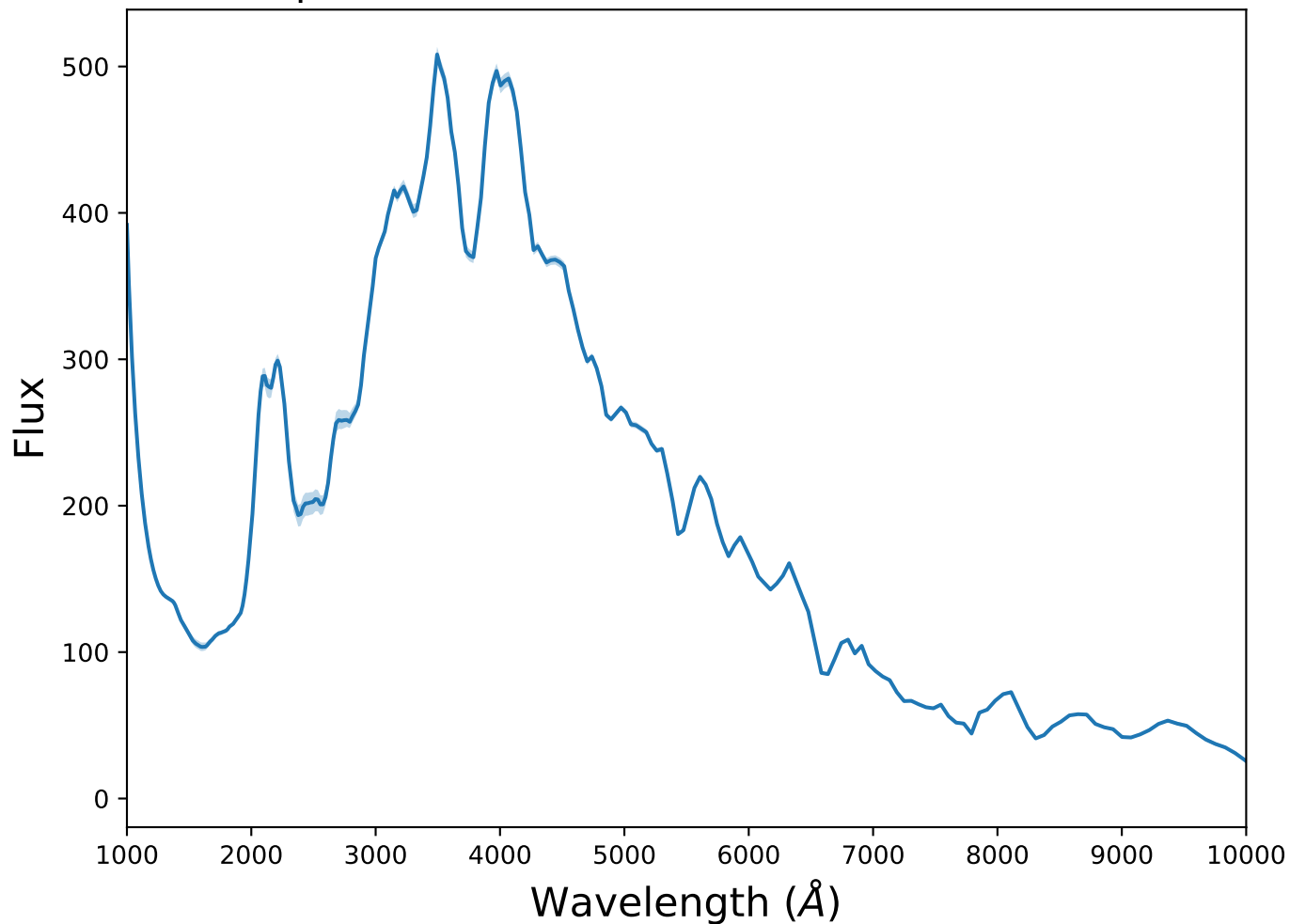
Spectrum 10 for transient SNIa at z=0.93
